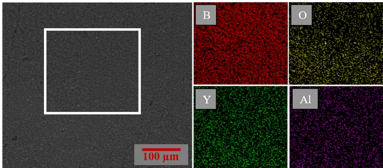
Figure 7. Elemental mapping of 3A-2Y precipitated sample sintered at 1800^\circ C
