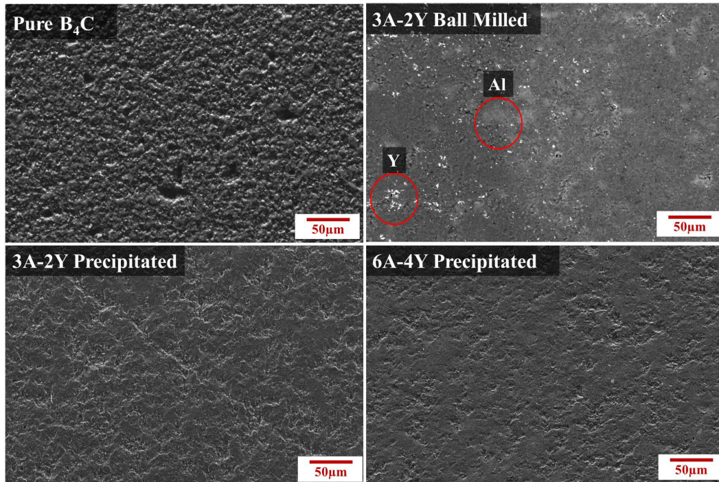
Figure 6. SEM images of pure, ball milled and precipitated B_4C at 1800^\circ C for 1 h
