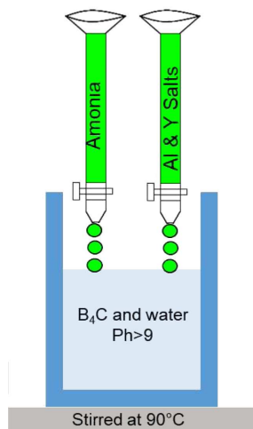
Figure 1. Illustration of precipitation setup
