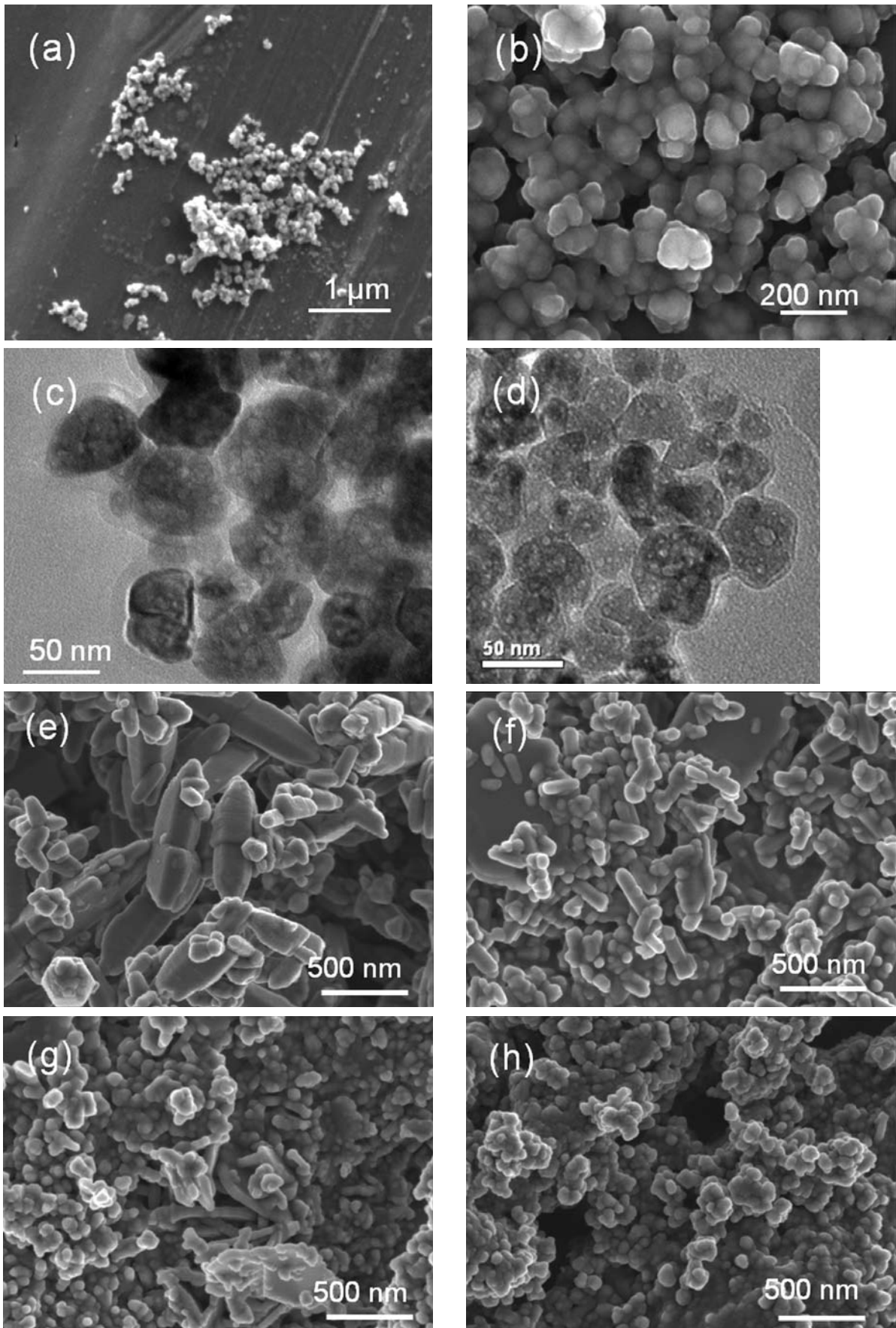
Figure 4. SEM and TEM micrographs of ZnO and Al-doped powders from different synthesis conditions (a,b,c) SFTR-A10-PAA, (d) SFTR-A10.005-PAA, (e) MW-A10, (f) MW-A10.05, (g) MW-A10.10, (h) MW-A10.05-PAA
